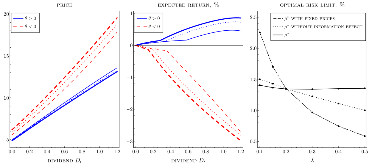
Figure 4: Comparative statics
